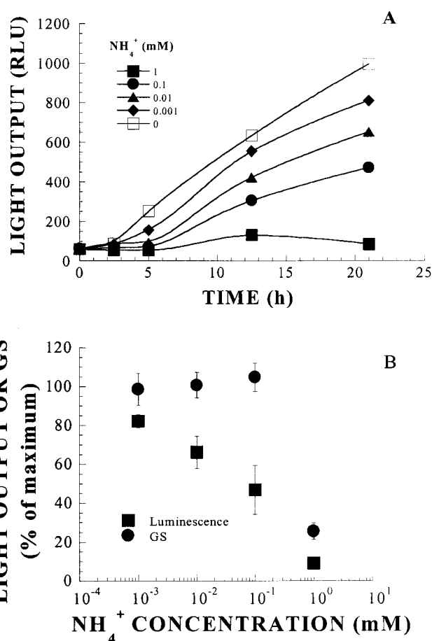
FIG. 2. Bioluminescence in Synechococcus sp. strain GSL. (A) Luminescence development in the presence of different \text{NH}_4^+ concentrations. (B) Light emission and GS activity as a function of \text{NH}_4^+ concentration following 20 h of exposure. Data in panel B (averages and standard deviations) represent the percent maximal luminescence or GS activity obtained at that time point in N-free medium in three replicate experiments ( 917.9 \pm 120.4 RLU or 443.4 \pm 34.0 \mu\text{mol of } \gamma\text{-GH h}^{-1} \text{ mg of protein}^{-1} , respectively).
