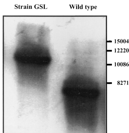
FIG. 1. Southern analysis of Apa I and Mfe I digests of genomic DNAs of wild-type Synechococcus sp. strain PCC7942 and strain GSL. The blot was hybridized with a fluorescein-labeled probe based on a 382-bp NSI PCR product. Numbers on the right indicate molecular weights.
