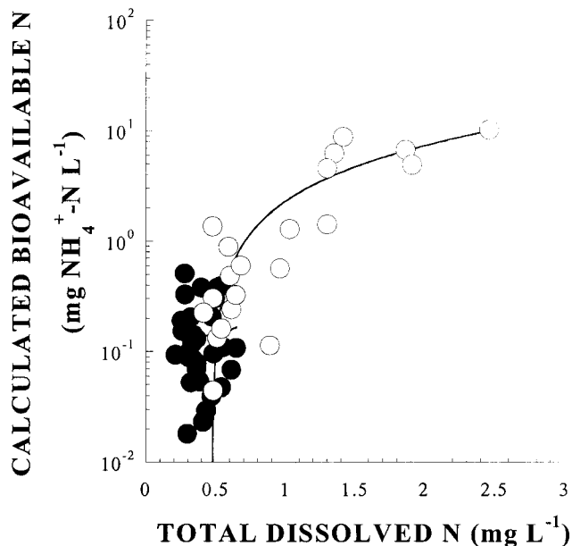
FIG. 8. Available N concentrations, calculated as ammonium equivalents and plotted as a function of TDN in the same samples. Symbols: ●, epilimnion samples; ○, hypolimnion samples.
